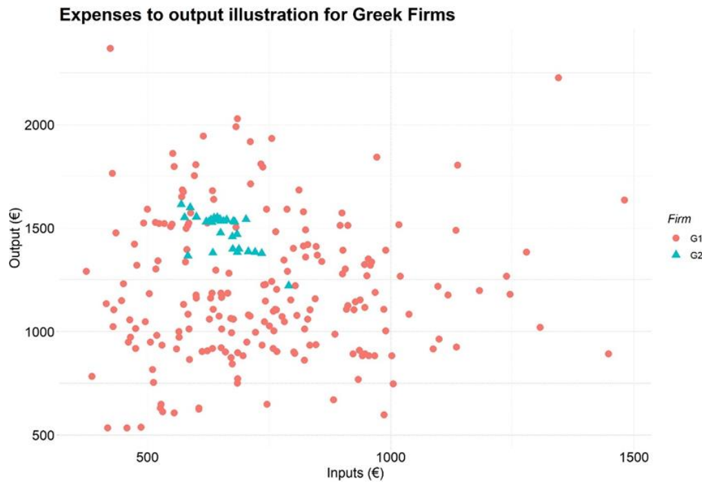
Figure 8. Monetary values of inputs used to final output for Greek firms.
