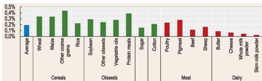
Figure 1. Change in agricultural commodity prices due to 1 percent increase in N, P, K fertilizer prices Source: OECD/FAO (2023), "OECD-FAO Agricultural Outlook", OECD Agriculture statistics (database), http://dx.doi.org/10.1787/agr-outl-data-en
